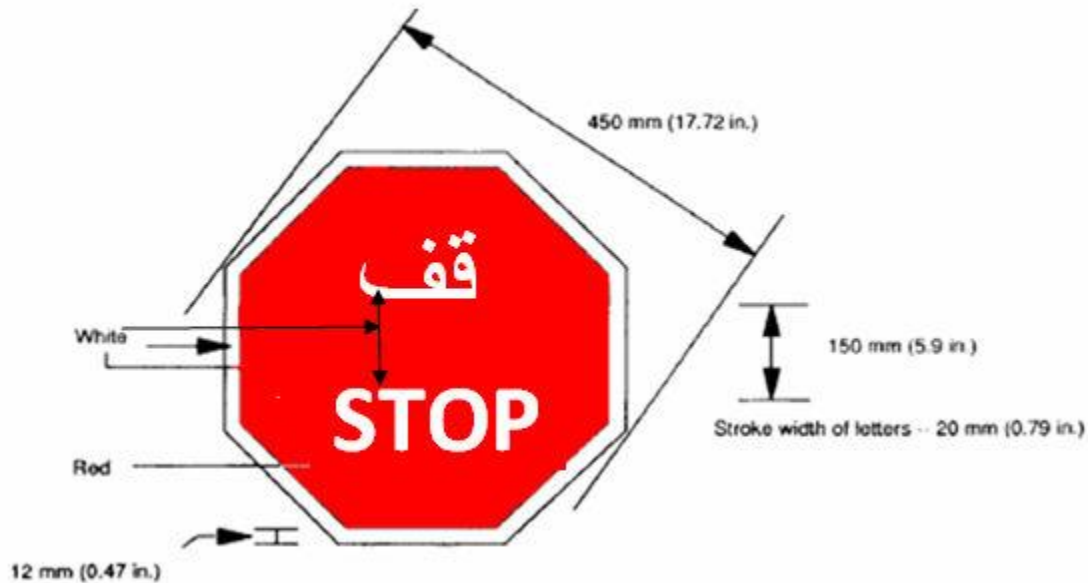
Figure 1: Stop arm
