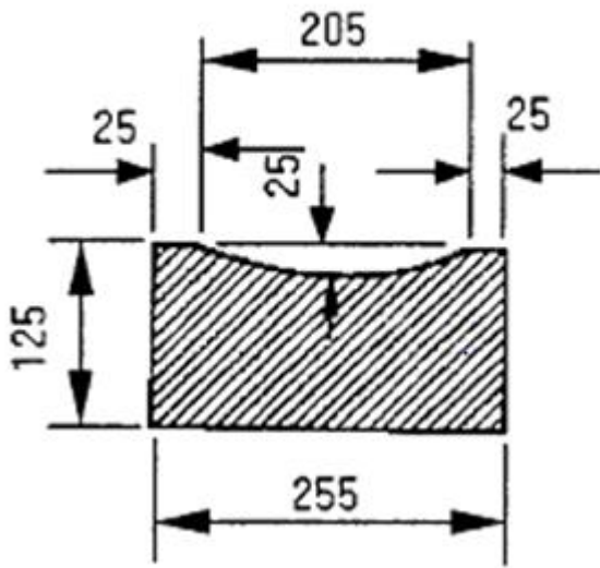
b) Channel dished : Type CD
